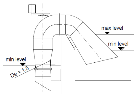
Axial, siphon 1.0 - 3.5 m
