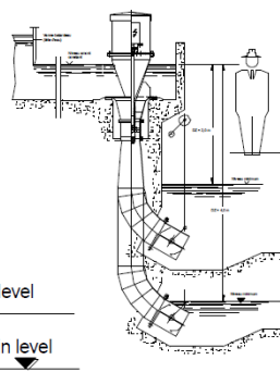
Axial, Pico turbine 1 - 5 m
