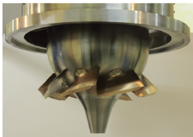
Diagonal Medium heads : 25 -100 m
